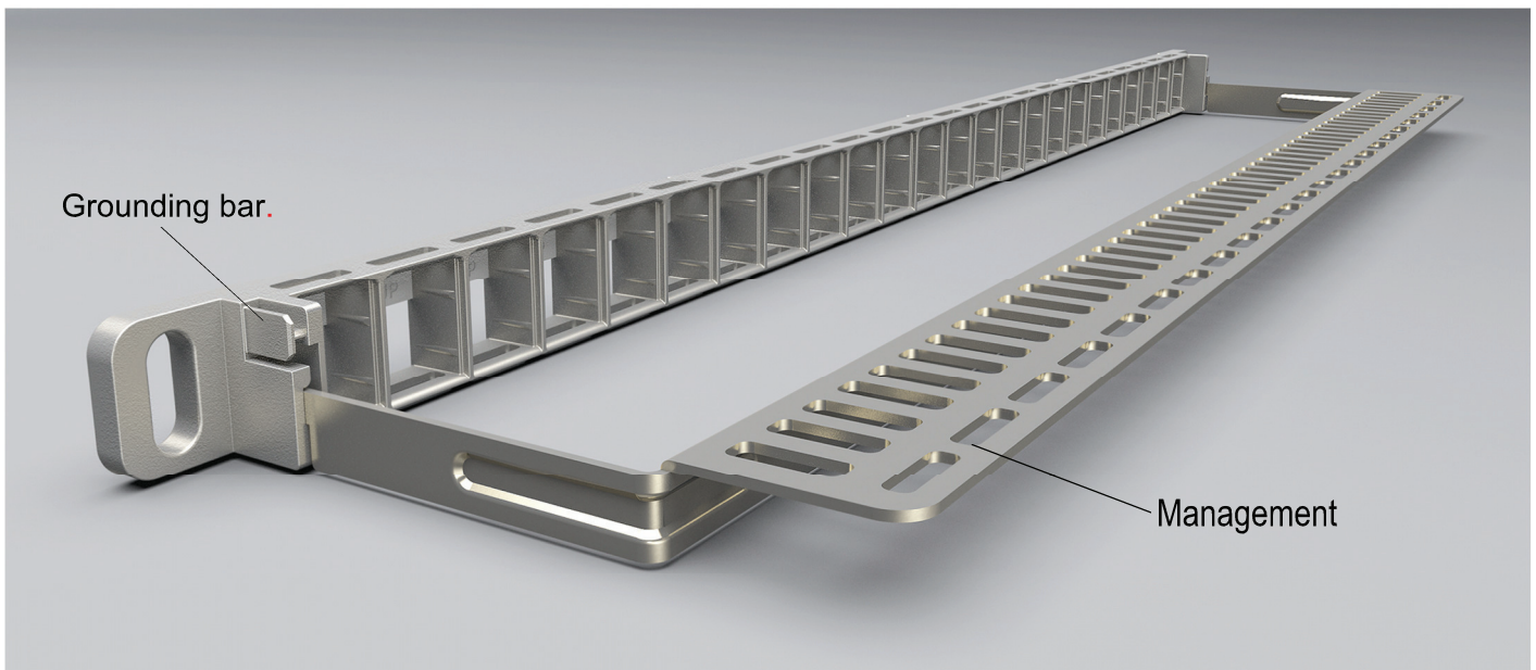
View of the assembled cable management frame.
