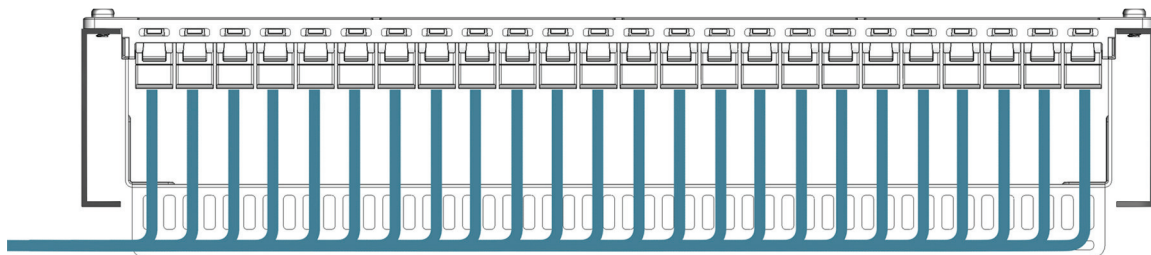
Figure 2: When all the cables are routed in one direction, they may be easily tie wrapped to the cable management at either of the cable management slots on the cable manager .
